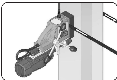
Wrap the safety belt around the work piece.
